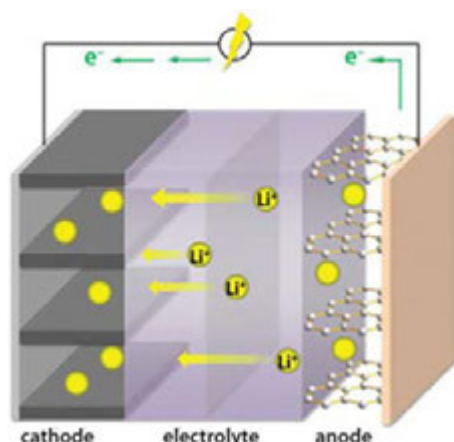
Figure 6.9. An electrochemical cell for the direct extraction of lithium ions from seawater. The cell is based on lithium-ion battery technology that has a high selectivity for lithium ions. Source: Used with permission from Kam and Doeff (2012)
